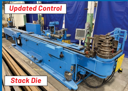
3" Schwarze-Robitec SW-60MW CNC Tube Bender
