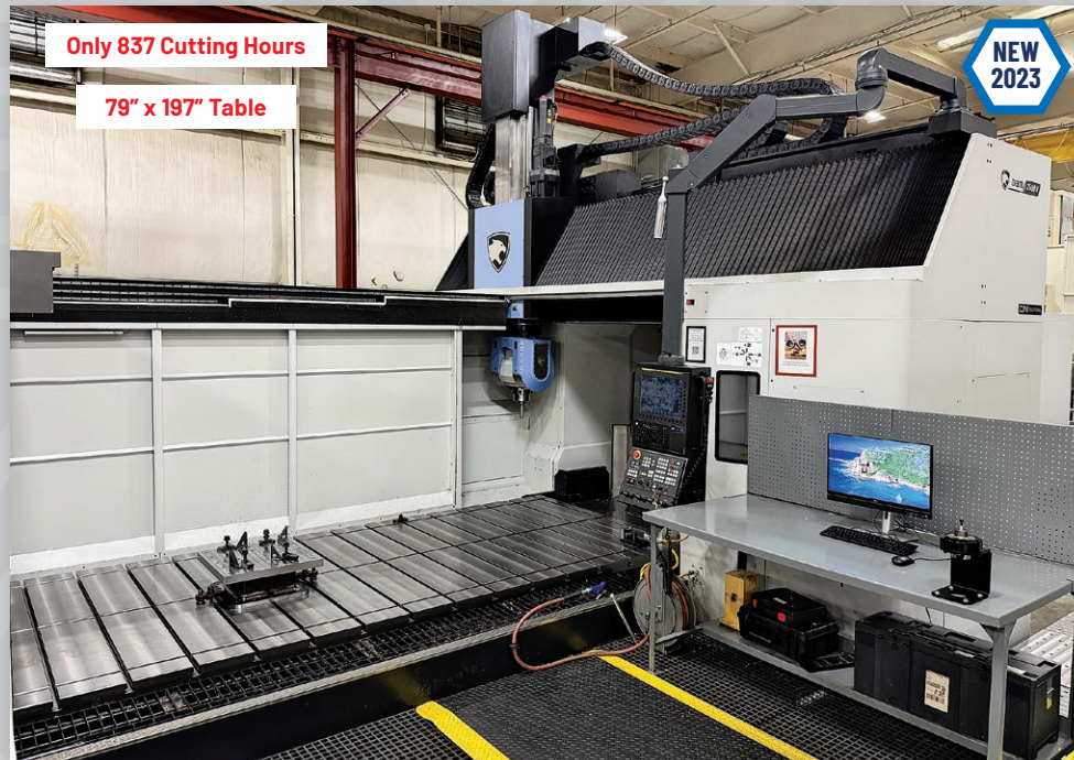
Doosan Model DBM 2550U Double Column Bridge Type CNC Five-Axis Machining Center (New 2023)
