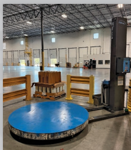
Cousins HP2100-SRT Stretch Wrapper
