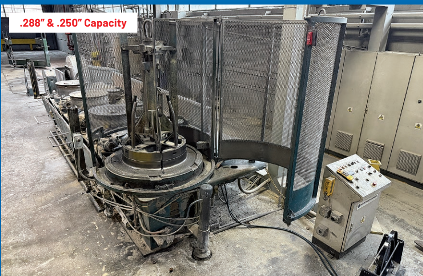
(3) Vaughn Motoblox and Ringblox Model 4/5 Wire Drawers, 27" Blocks / 30" Finishing Block
